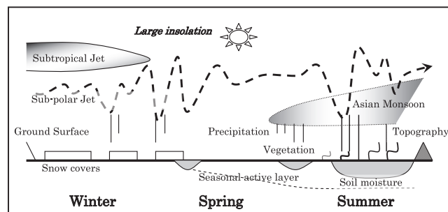
Figure 2. Land-atmosphere interactions, convective activity, and onset of Asian Monsoon (courtesy of Kenichi Ueno, University of Tsukuba).
