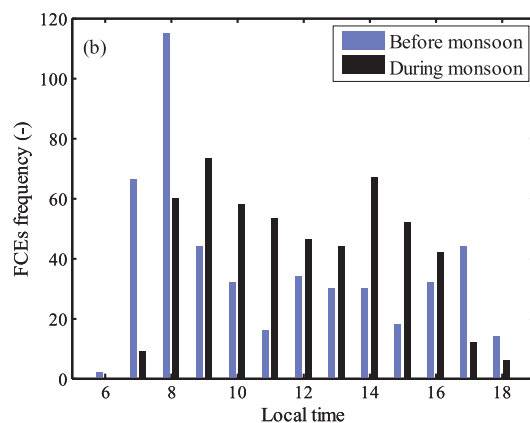
Figure 4. Observed Free Convection Events: Before the monsoon, FCEs mostly occur in the morning hours. During the monsoon, the distribution is bi-modal with an afternoon mode closely related with cloud cover (courtesy of Kenichi Ueno, University of Tsukuba, Japan).
