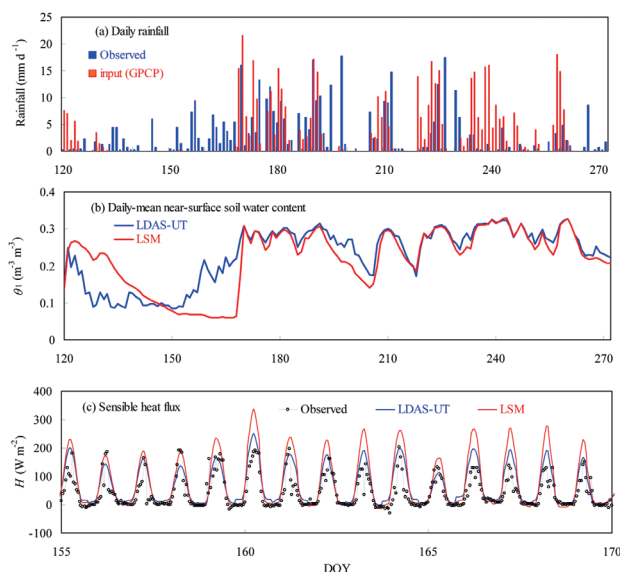
Figure 4. (a) Daily mean precipitation in terms of both measurements and LDAS-UT/LSM input (GPCP), (b) Daily mean near-surface soil water content estimated by LDAS-UT and LSM (SiB2), and (c) Surface sensible heat fluxes derived from LDAS-UT and LSM (SiB2) for the CEOP East Tibet site. DOY is 2003.
