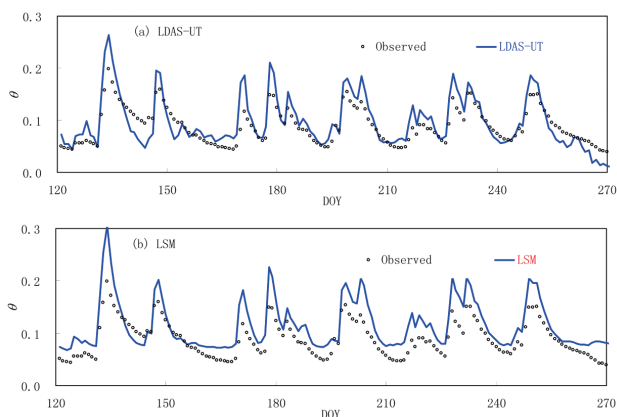
Figure 3. Comparisons of AMPEX daily-mean station-averaged near-surface soil volumetric water content with (a) LDAS-UT output, and (b) LSM (SiB2) simulation at the CEOP Mongolian site during 30 April 2003 to 30 September 2003.
