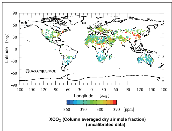
The CO 2 column averaged dry air mole fraction distribution. Data are excluded where the associated radiance spectra are saturated and where noise is relatively large due to weak ground surface reflection.
