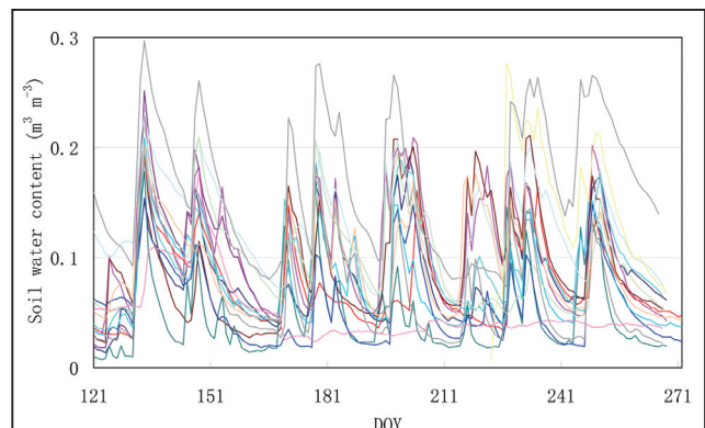
Figure 2. Observed daily-mean near-surface (3 cm depth) soil moisture variations at 16 Mongolian AMPEX stations during the period of 30 April 2003 to 30 September 2003.
