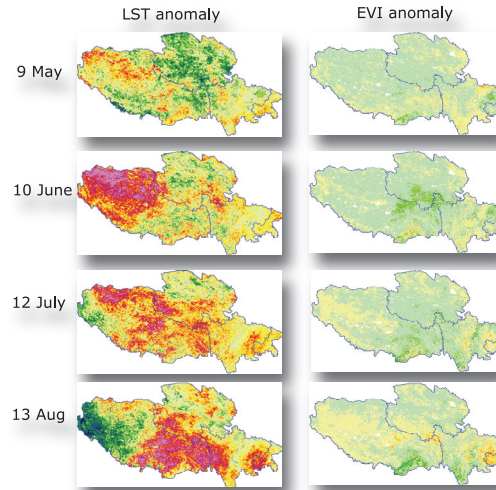
Figure 6. Early detection of drought by time series analysis of LST and EVI MODIS data (Courtesy of L. Jia, Wageningen University and Research Centre, The Netherlands).
