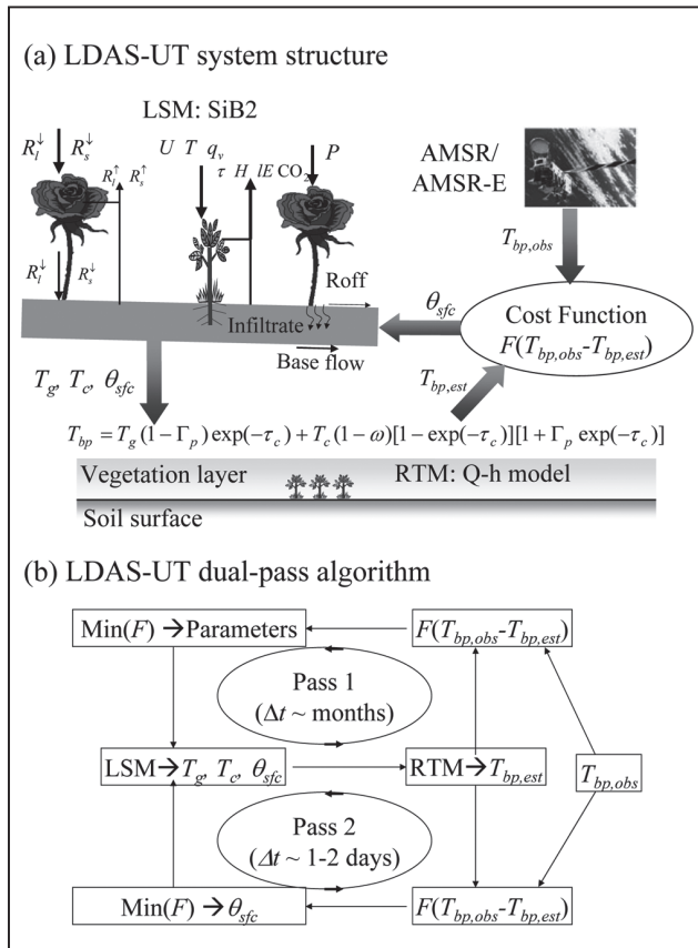
Figure 1. (a) LDAS-UT system structure and (b) schematic of the dual-pass assimilation technique. T_g , T_c , and \theta_{sfc} are the ground temperature, canopy temperature, and near-surface soil water content, respectively. T_b is the brightness temperature, F the cost function, and \Delta t the data assimilation window. \Gamma_p is soil reflectivity, \tau_c the optical thickness of the vegetation. The subscript p denotes the polarization, obs the observed value, and est the estimated value (Yang et al., 2007).
