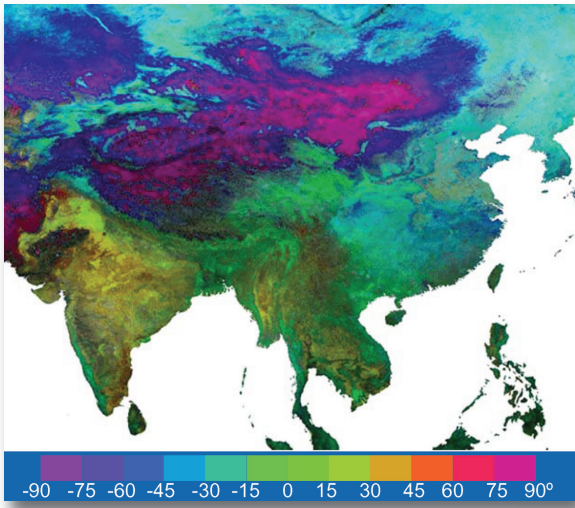
Figure 5. Correlation of yearly amplitudes of Land Surface Temperature vs. NDVI over the period 2000 - 2006; positive angles indicate positive correlation of LST and NDVI (courtesy of J.A.Sobrino, University of Valencia, Spain).
