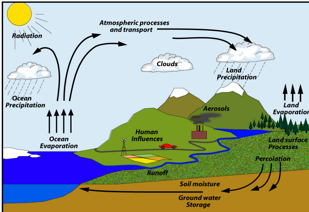
Fig. 1 depicts the hydrological cycle schematically and thus the driving by radiation and energy, the atmospheric dynamics that move water and energy around and produce clouds which block the sun, the complex land surface complete with human influences and the interactions with the atmosphere, and the surface and below surface processes that complete the water cycle (adapted from Trenberth et al. 2007).
